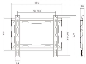
Dimensions (mm)
